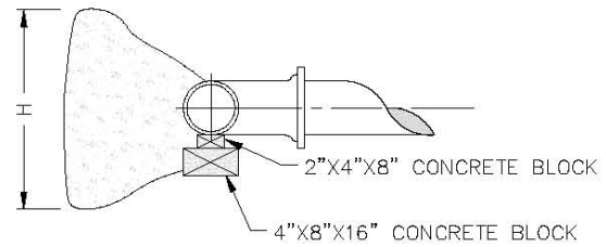
TYPICAL SECTION NOT TO SCALE
