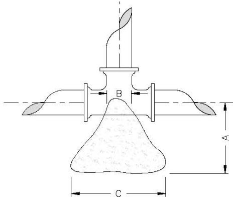
TEES AND TAPPING SLEEVE NOT TO SCALE
